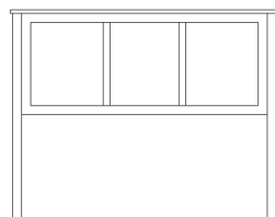
FULL PANEL HEADBOARD 141-20-1001 58 x 3 x 46 in
